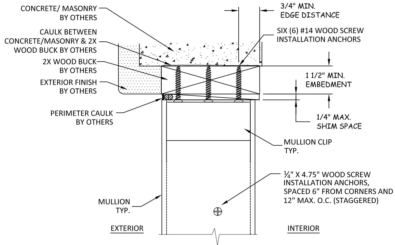
B 4 VERTICAL SECTION HEAD - 2X WOOD BUCK CLIPPED TUBE MULL
