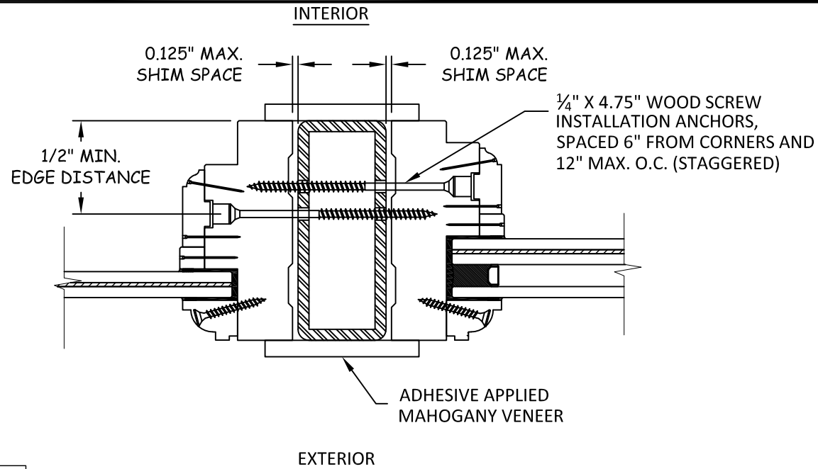
F 5 HORIZONTAL SECTION 1/4" X 2" X 5" ALUMINUM TUBE MULLION
