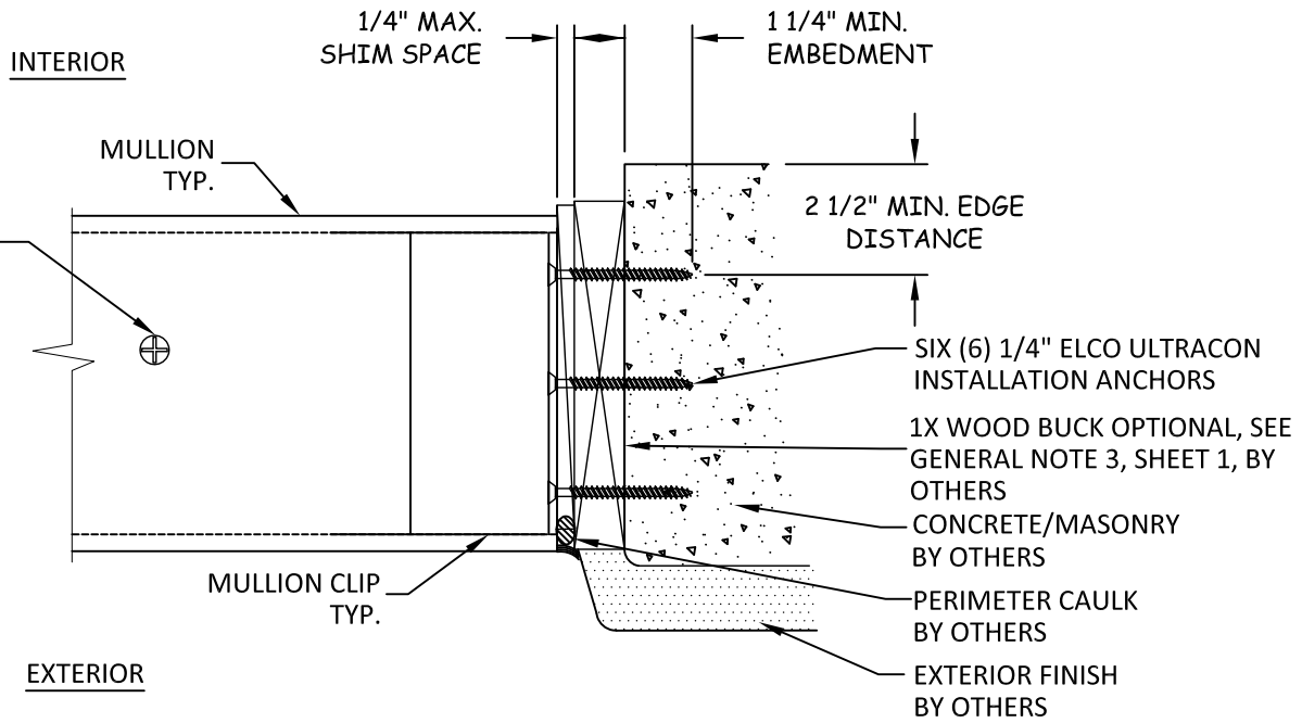
I 6 HORIZONTAL SECTION JAMB - CONCRETE/MASONRY CLIPPED TUBE MULL
