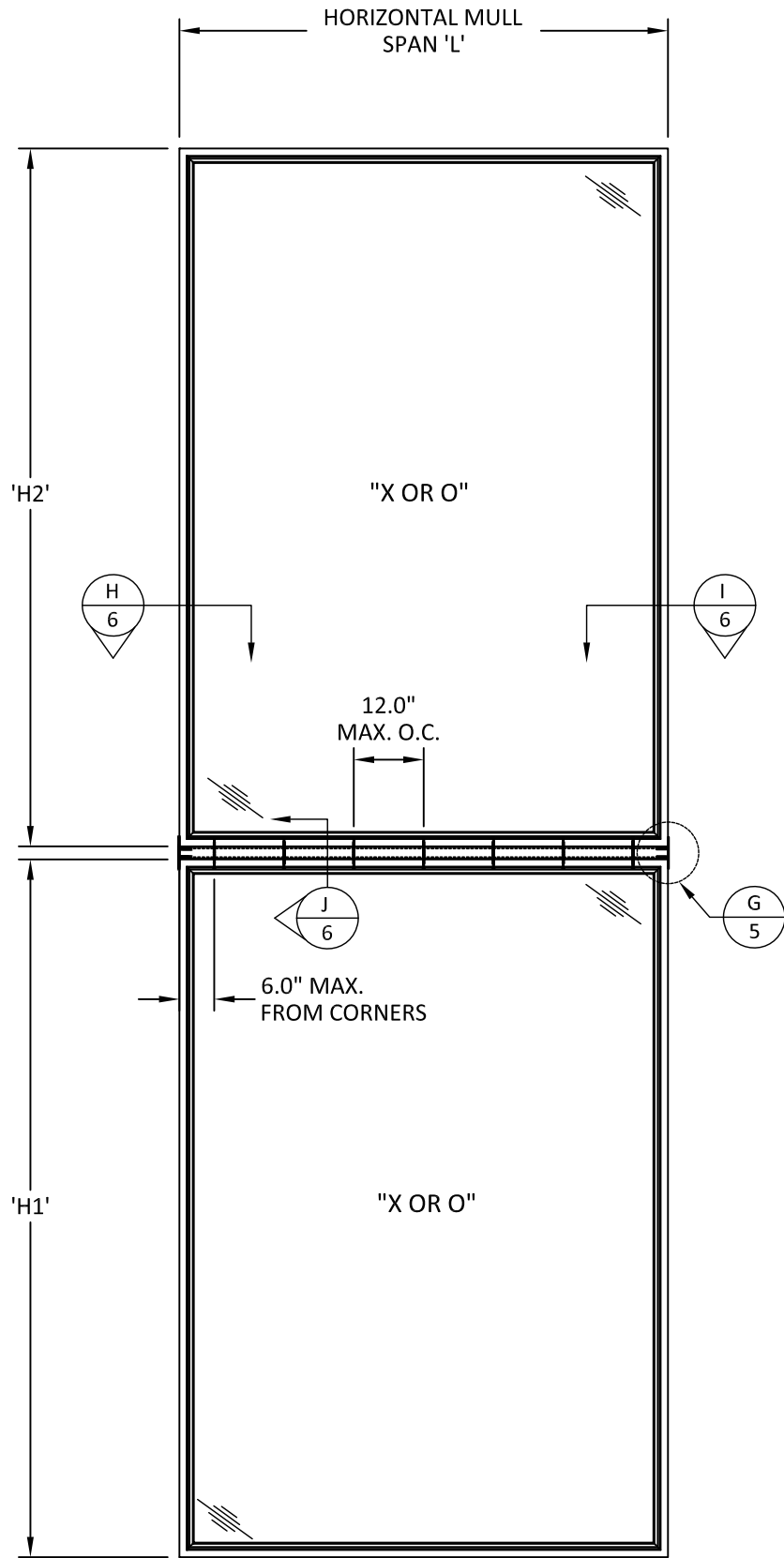
TYPICAL MULLION ASSEMBLY 1/4" x 2" x 5" CLIPPED HORIZONTAL ALUMINUM TUBE MULLION
